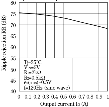
Fig.15 Ripple Rejection vs. Output Current (PQ20WZ11)
